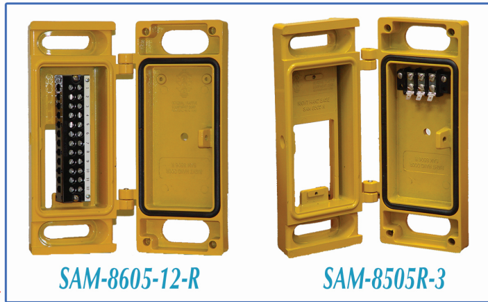
Swing Arm Mount Assembly, "Clamshell" style for PED Signal Mounting, Three & Twelve Position Terminal Block, Set of Door & Base.
